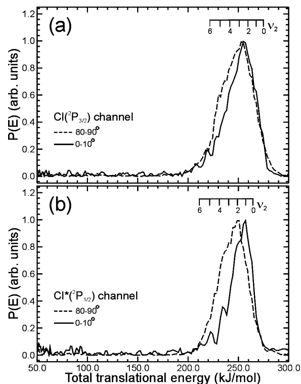
Figure 4. Normalized translational energy release distributions for photofragment ejection in two different angular regions following the 193.3 nm photolysis of CH 3 Cl. (a) Cl ( ^2P_{3/2} ) channel. (b) Cl* ( ^2P_{1/2} ) channel. The positions of the CH 3 \nu_2 vibrational combs should only be regarded as a qualitative guide to the extent of any internal excitation, as discussed in the main text.
